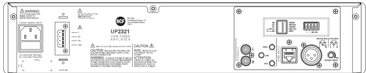
Rear panel
