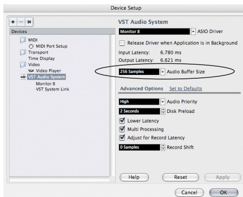
Figure 7-5: In Cubase or Nuendo, choose Devices menu > Device Setup. Select your interface (Monitor 8), then click the Control Panel button to access the window above and the Buffer Size setting.
