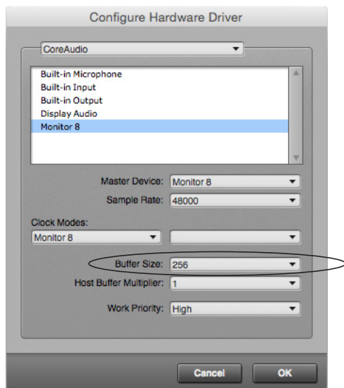
Figure 7-4: In Digital Performer and AudioDesk, choose Setup menu > Configure Audio System > Configure Hardware Driver to open the dialog shown above and access the Buffer Size setting. Refer to your Digital Performer or AudioDesk manual for information about the Host Buffer Multiplier setting.
